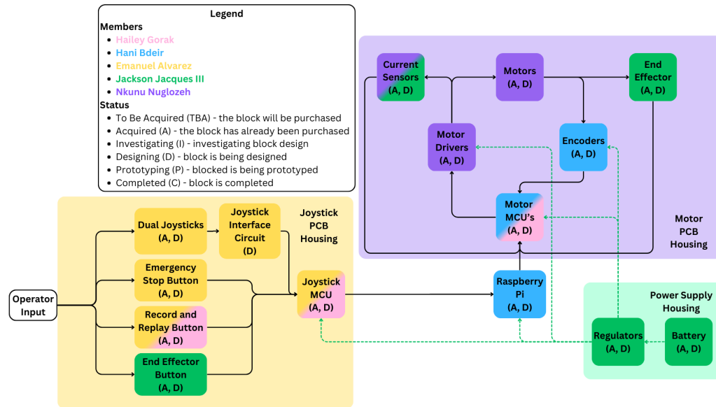
Figure 2.5.1 - Hardware Block Diagram
